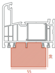
U=0,70 W/m 2 K Gealan S8000 iQ, S9000 iQ
