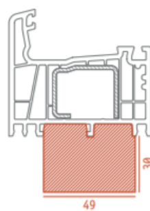
U=0,79 W/m 2 K Salamander Streamline, SL76, 3D
