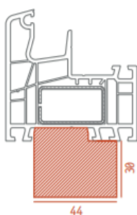
U=0,88 W/m 2 K Aluplast Ideal 5000, Ideal 4000
