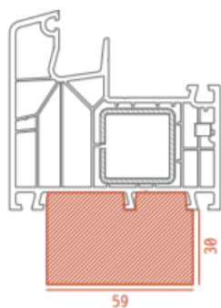
U=0,66 W/m 2 K Aluplast Ideal 8000, Ideal 7000
