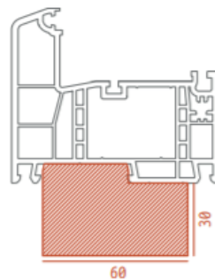
U=0,65 W/m 2 K Rehau Geneo
